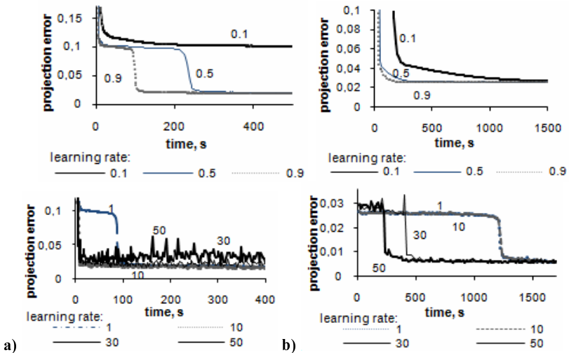
Fig 4. The dependence of the projection error on the computation time for the salinity dataset (a) and the iris dataset (b)
